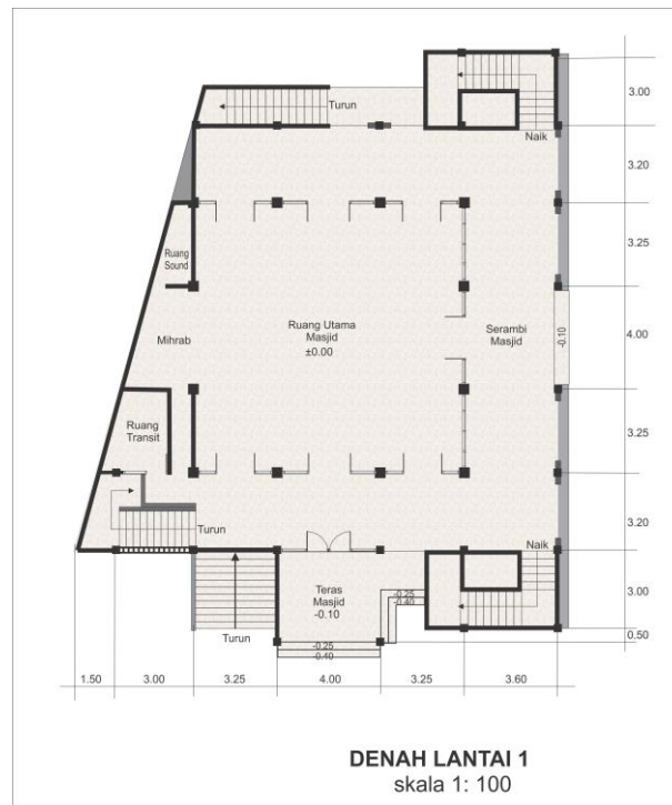
Gambar 5.1. Denah Lantai I Masjid As Salam
