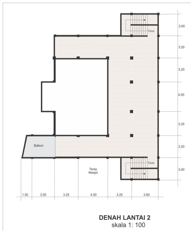
Gambar 5.2. Denah Lantai II Masjid As Salam
